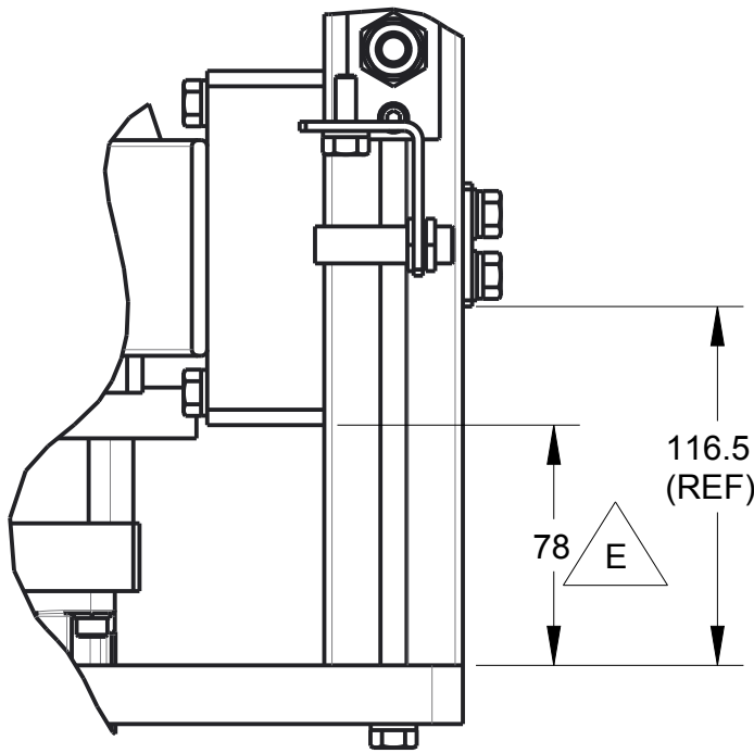
AUXILIARY VIEW SCALE 3/8
